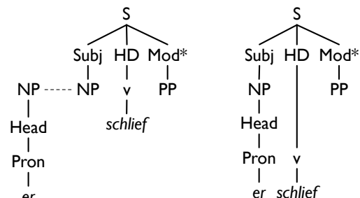
Figure 1. LEFT: Binding (dashed line) of lexical frames associated with er and schliefe . RIGHT: Derived tree.
